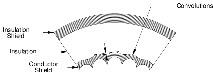
Figure 9-2 Procedure to Measure Irregularities
