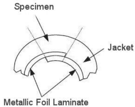
Figure 9-4 Example of overlapped metal foil (Not to scale)
