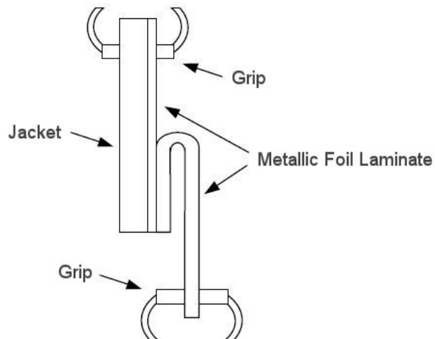
Figure 9-5 Peel strength of overlapped metal foil (Not to scale)
